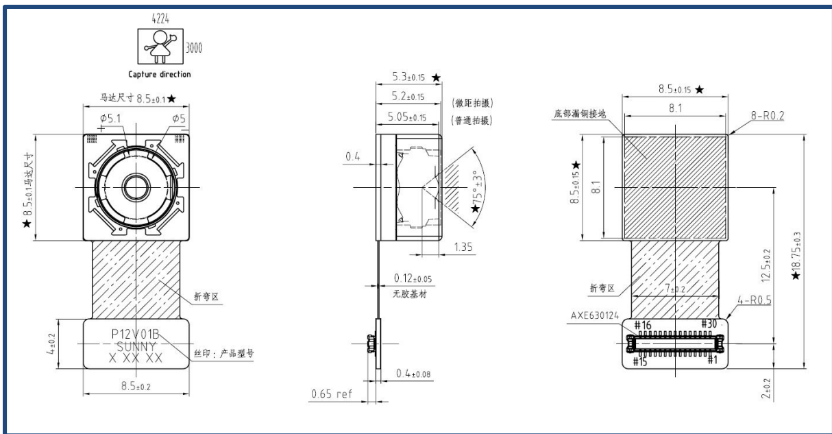
Figure 1: Mechanical Drawing
